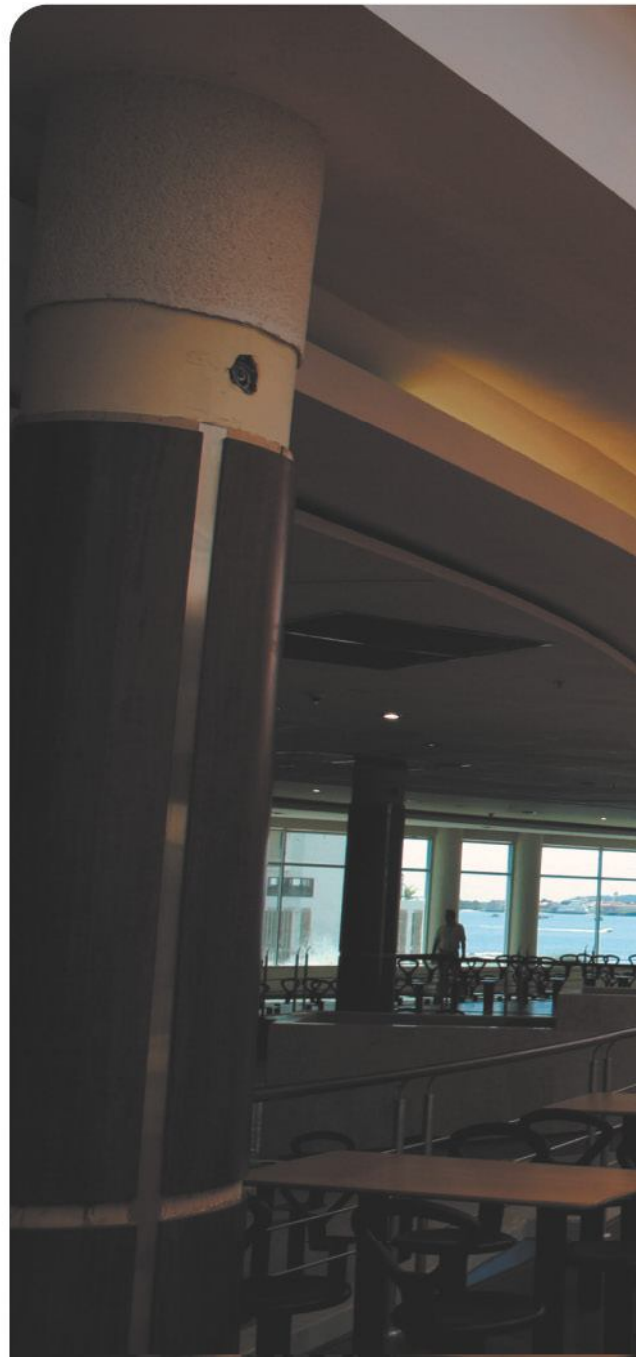
Muticentro Mall, Panama 8 mm Ice Polygal Sheets, HCP connection system
